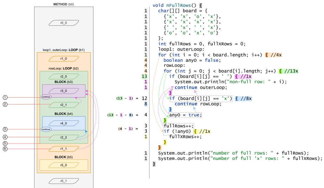
Figure 4.5: A program with control flow breaks and calculated region hit-counts
