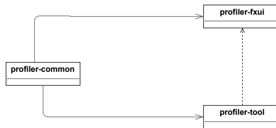
Figure 4.2: The project’s Java module dependencies. The fxui and tool modules both depend on the common module. fxui only uses the tool when executing its main method, but does not depend on any other implementations of it.
