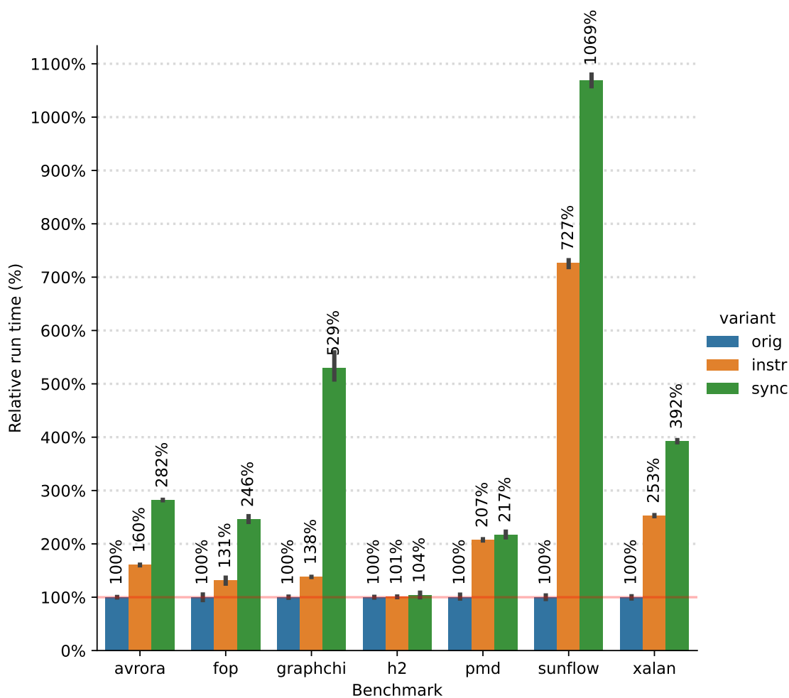
Figure 6.1: Relative run-time overhead of our profiler applied to DaCapo benchmarks, using synchronized and unsynchronized counter variants
