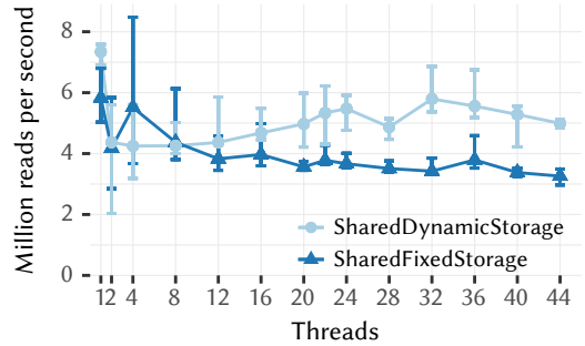
Fig. 7. Throughput of array reads when migrating 1000 SharedFixedStorage arrays every 5 seconds compared to starting with SharedDynamicStorage.
